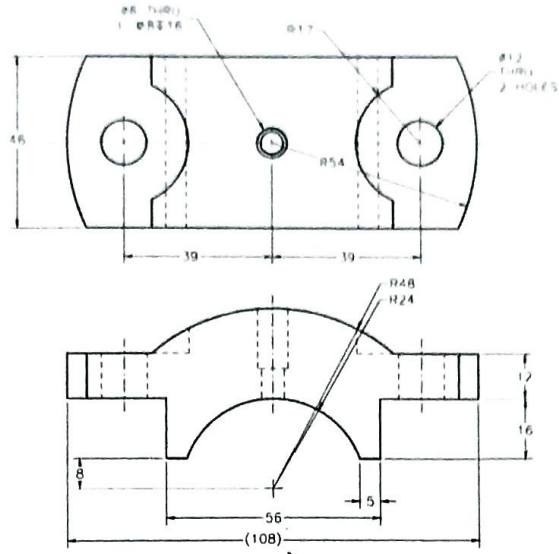
Figure 3 Views and dimensions of the Cap
