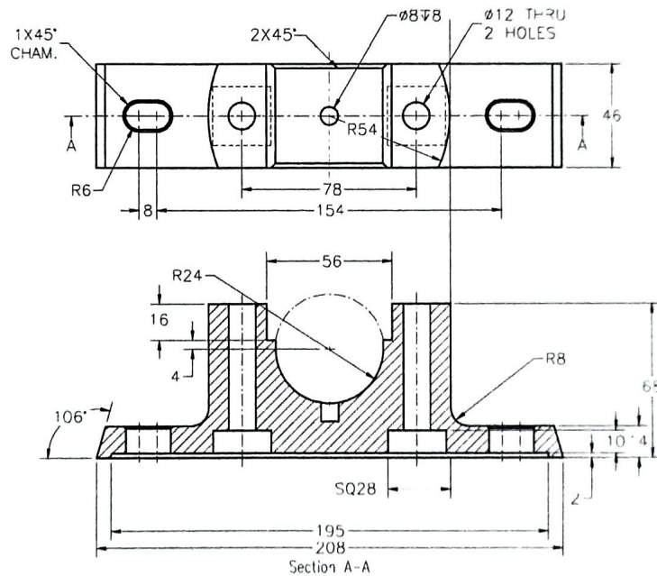
Figure 2 Views and dimensions of the Casting
